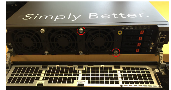
FIGURE 2 Loosen the two thumb screws (circled in red) that secure the fan module
